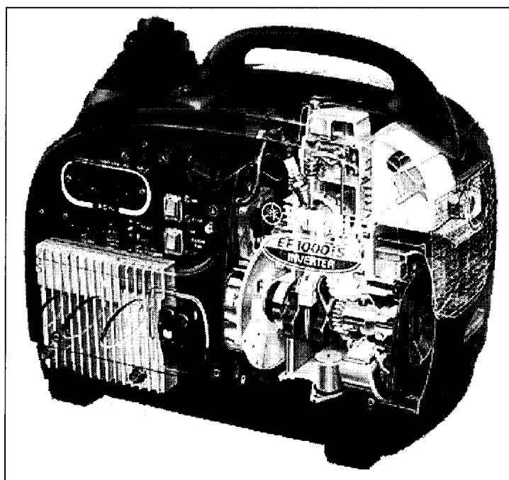
Design Schematic
